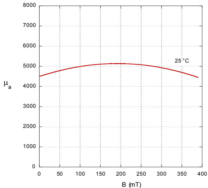
Amplitude Permeability vs. Flux Density
