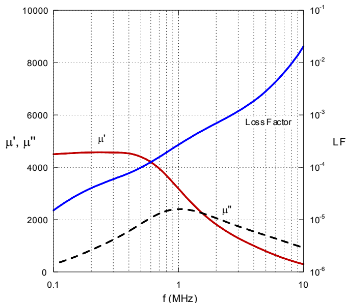
Permeability & Loss Factor vs. Frequency
